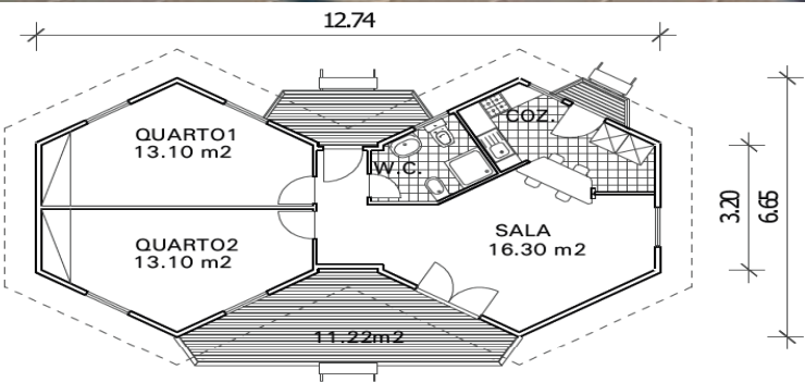
PLANTA T2 65 65.00 m2
